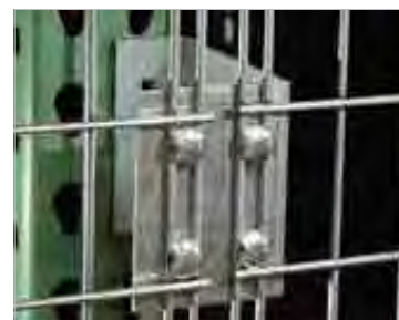
Offset brackets are available in different distances
